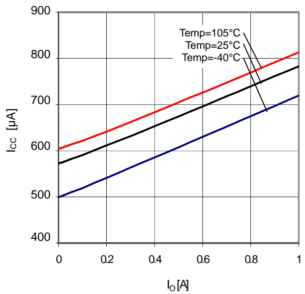
Figure 30. I_o-I_{cc}
