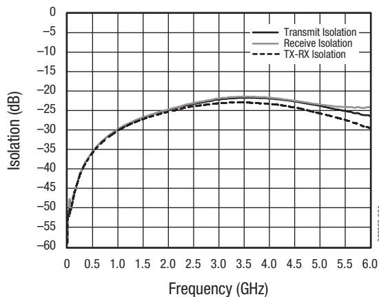
Figure 4. Typical Isolation
