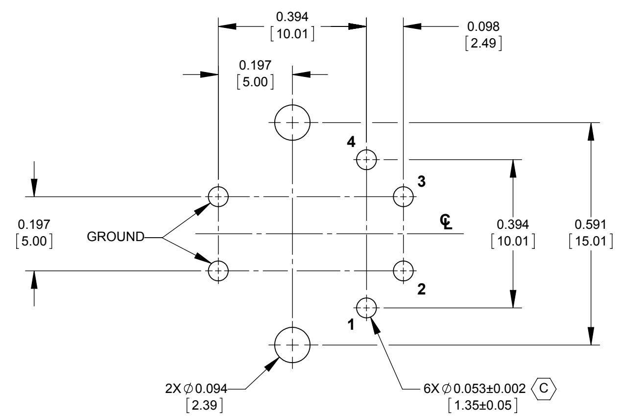
RECOMMENDED PC BOARD LAYOUT COMPONENT SIDE
