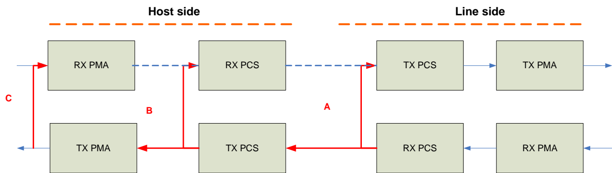
Figure 26: Line-side Loopback
