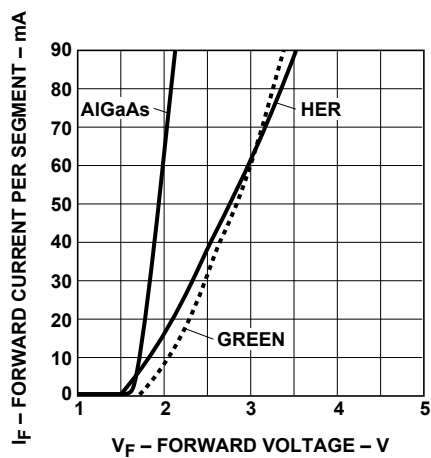
Figure 2. Forward Current vs. Forward Voltage.
