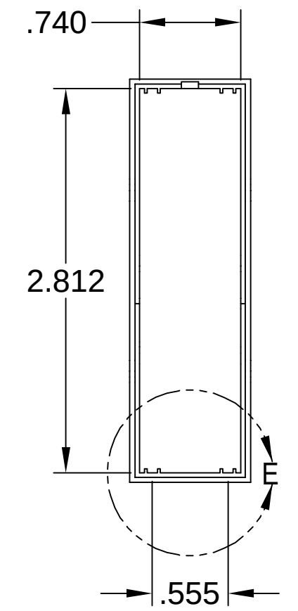
SECTION C-C
