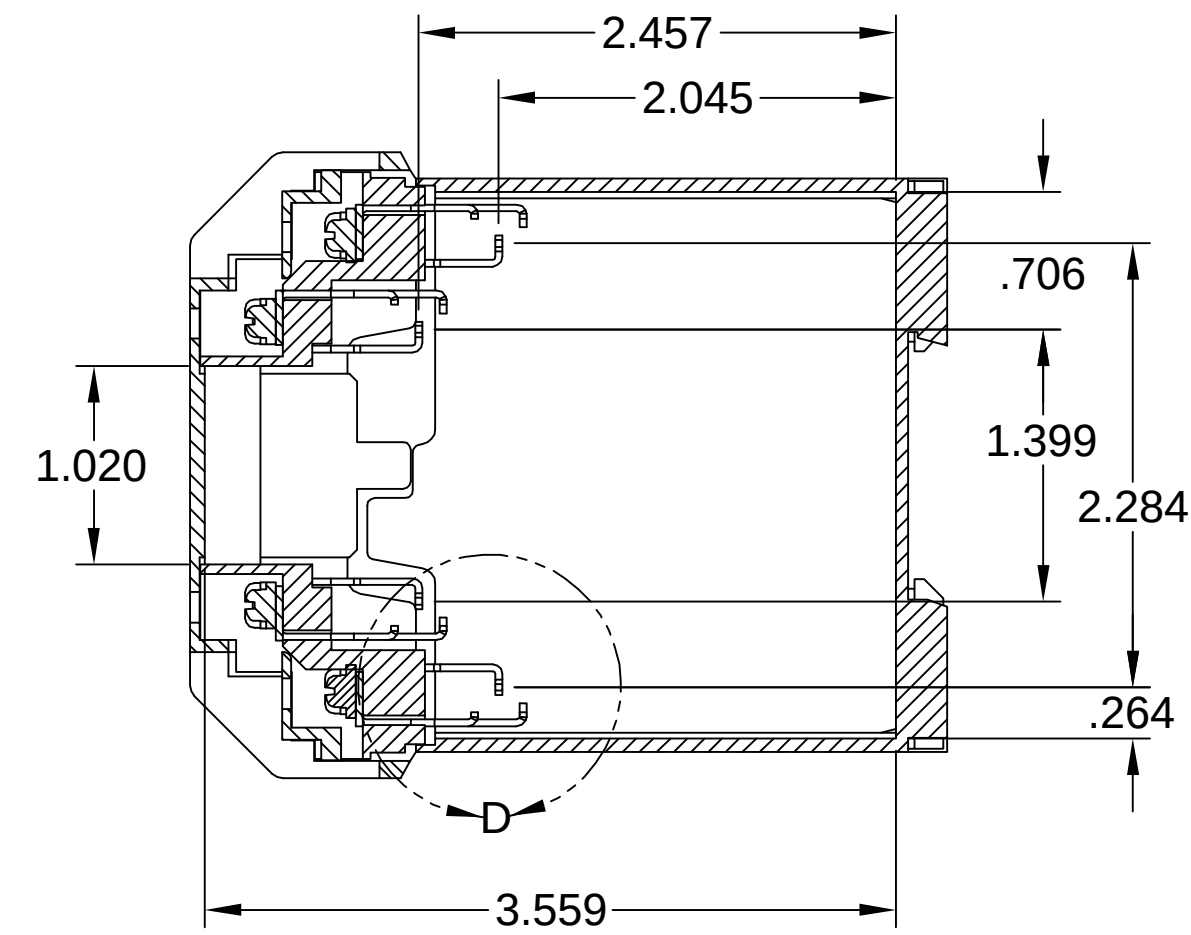
SECTION B-B
