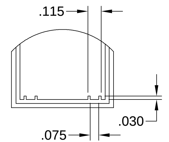
DETAIL E
