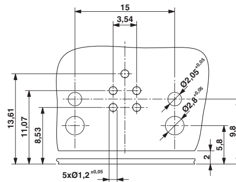
Drilling diagram only valid in connection with the SACC-M12-SCO PLUG L90 housing (order no. 1436709)
