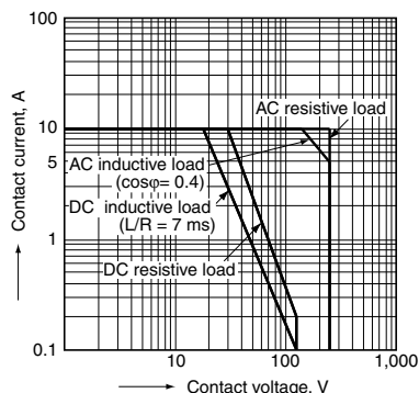
1-(1). Maximum operating power (1 Form A)
