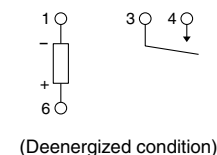
Schematic (Bottom view) Single side stable type
