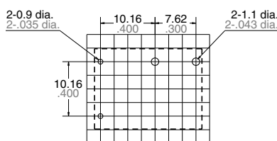
PC board pattern (Bottom view) Single side stable type
