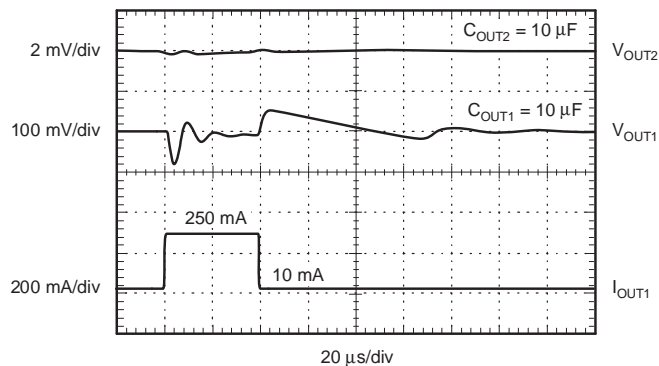
TPS71256 LOAD TRANSIENT RESPONSE AND V OUT2 CROSSTALK
