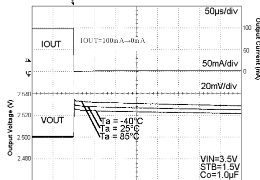
Fig. 79 Load Response
