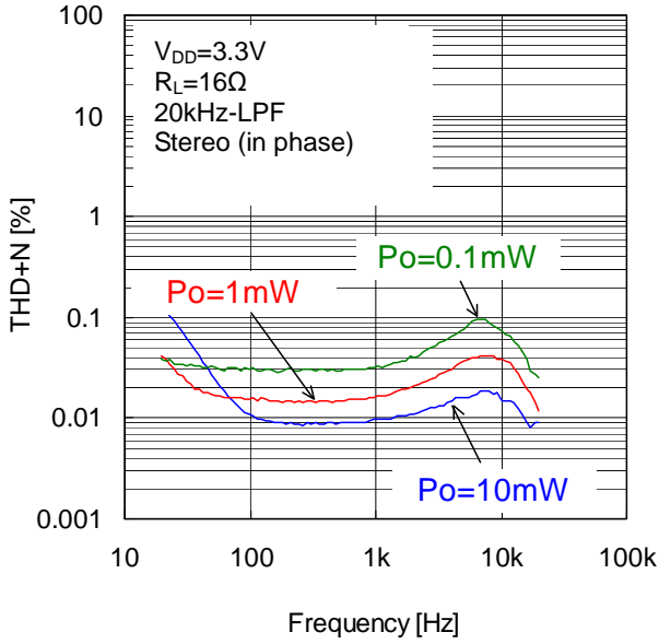
Figure 17. THD+N vs Frequency (V DD =3.3V, R L =16Ω)
