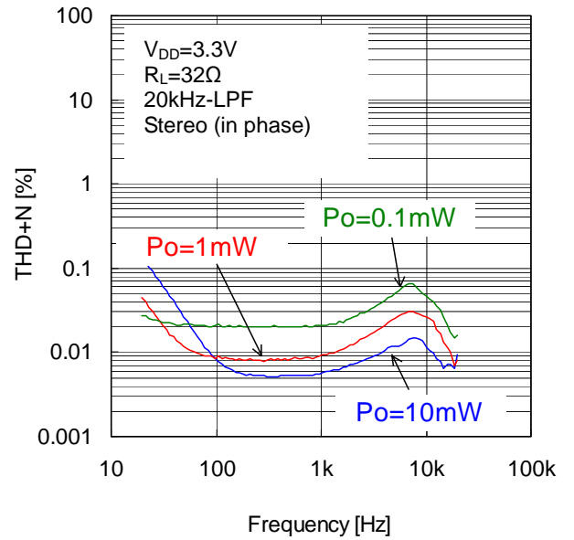
Figure 18. THD+N vs Frequency ( V_{DD}=3.3V , R_L=32\Omega )
