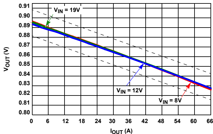
FIGURE 1. LOAD LINE REGULATION
