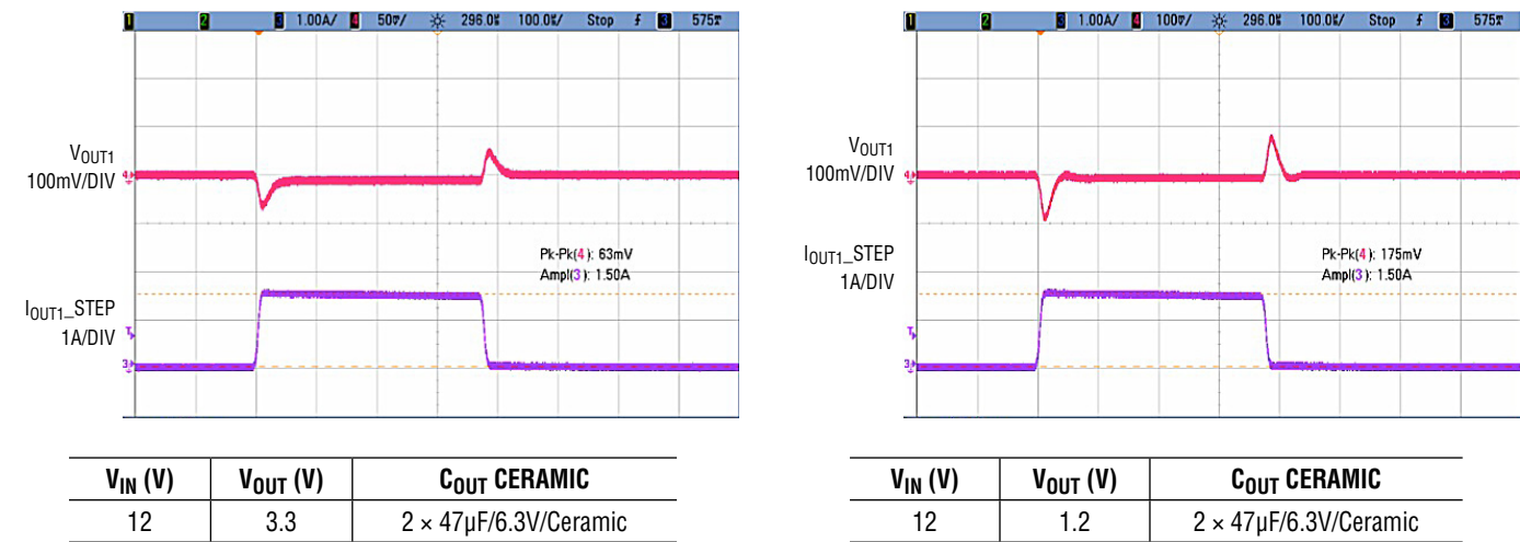
Figure 3. Measured V OUT1 = 3.3V and V OUT4 = 1.2V Load Transient Responses (1.5A to 3A Load Step)
