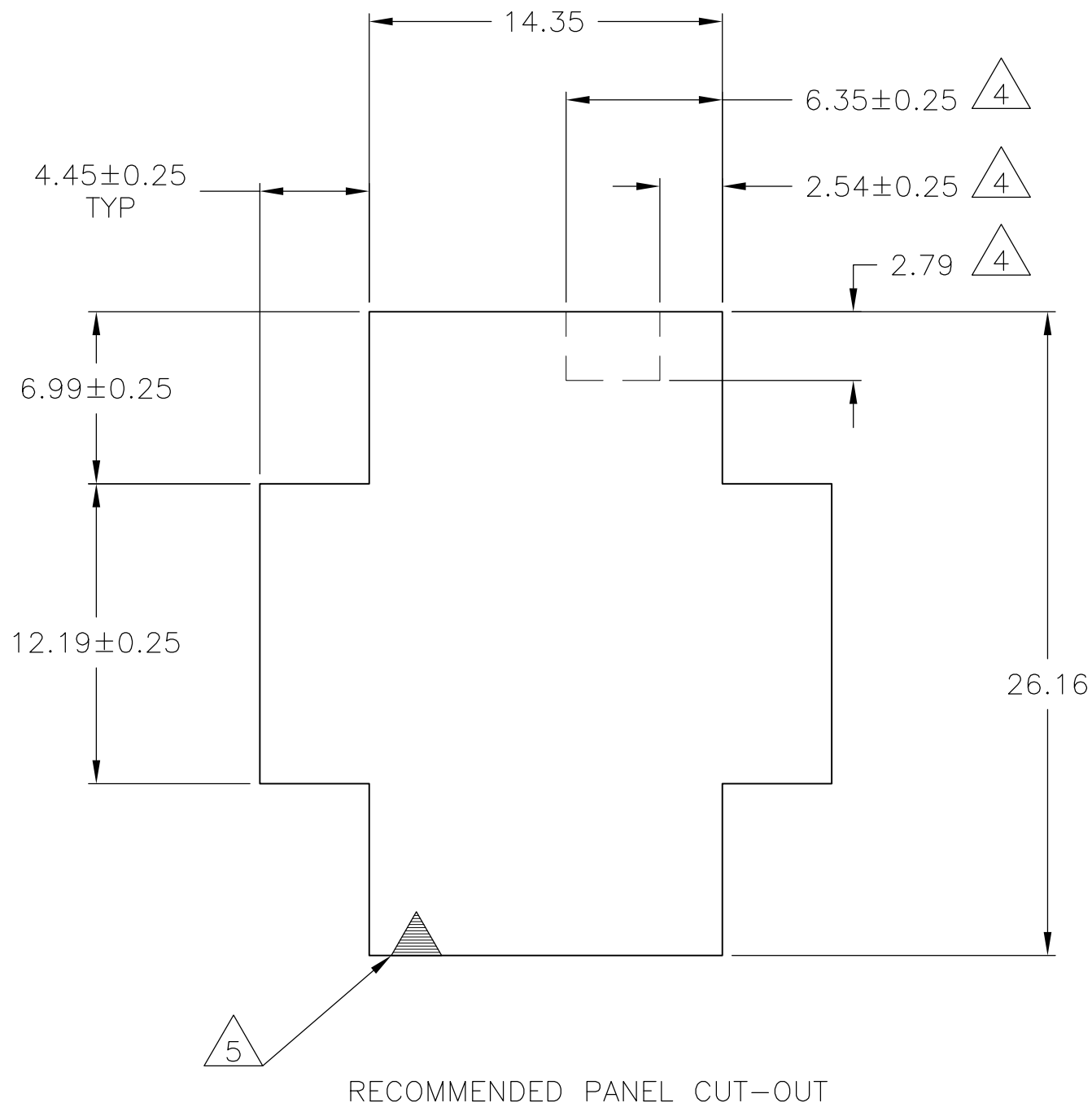
RECOMMENDED PANEL CUT-OUT
