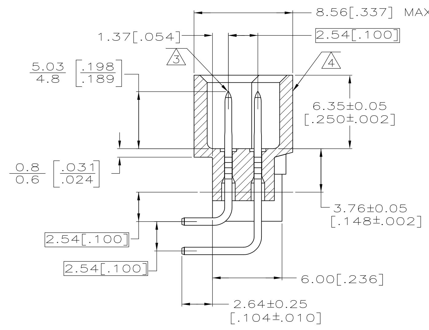
SECTION X-X
