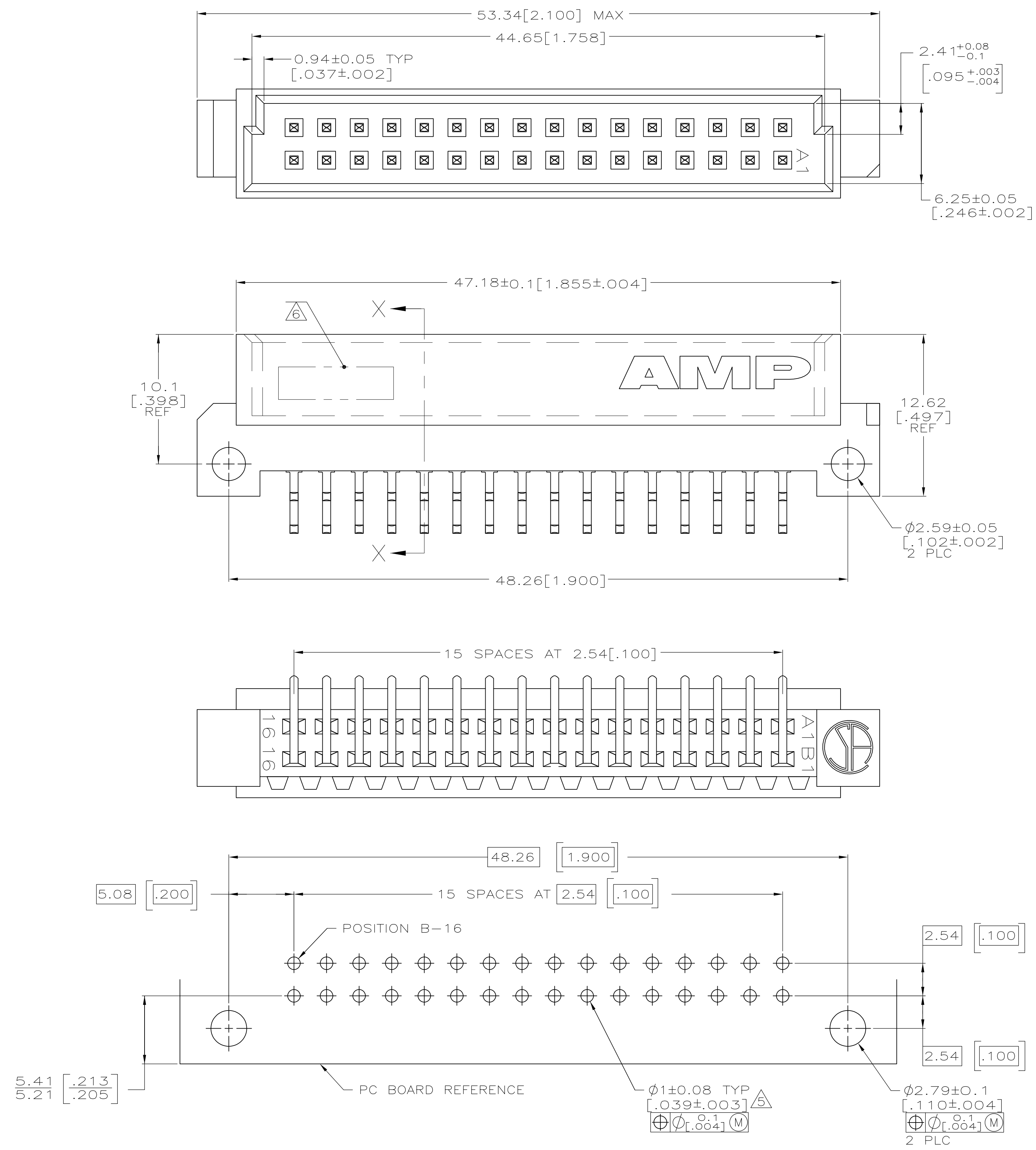
PC BOARD LAYOUT
