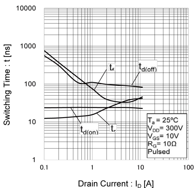
Fig.15 Switching Characteristics
