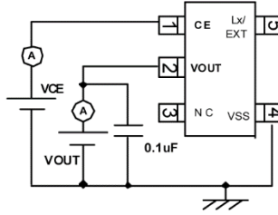
Circuit ⑥
