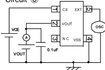
Circuit ⑧
