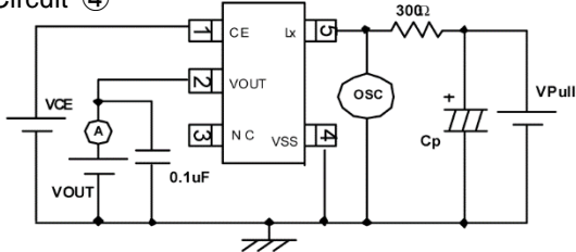
Circuit ④
