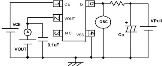
Circuit ④
