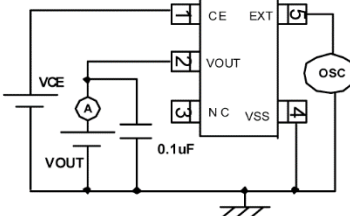
Circuit ⑧
