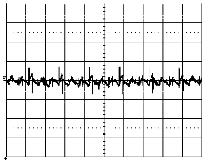
Output voltage ripple (20 mV/div.) at: T_{ref} = +25^\circ\text{C} , I_o = 50\text{ A} resistive load, V_i = 12.0\text{ V} . Time scale: 2 \mu\text{s}/\text{div} . See the filter in the Output ripple and noise section (EMC Specification).
