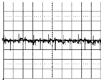
Output voltage ripple (20 mV/div.) at: T_{ref} = +25^\circ\text{C} , I_o = 50\text{ A} resistive load, V_i = 12.0\text{ V} . Time scale: 2 \mu\text{s}/\text{div} . See the filter in the Output ripple and noise section (EMC Specification).
