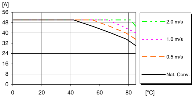
Available load current vs. ambient air temperature and airflow at V_i = 12.0 V, V_{OUT} = 1.2 V . See Thermal Consideration section.
