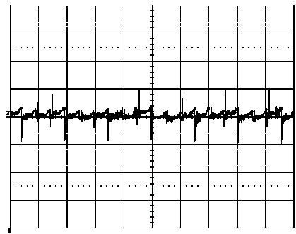
Output voltage ripple (20 mV/div.) at: T_{ref} = +25^{\circ}C , I_o = 50 A resistive load, V_i = 12.0 V. Time scale: 2 \mu s/div. See the filter in the Output ripple and noise section (EMC Specification).
