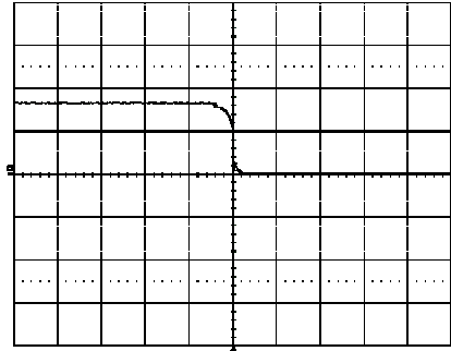
Shut-down enabled by disconnecting V_i at: T_{ref} = +25^{\circ}C , I_o = 50 A resistive load, V_i = 12.0 V. Top trace: output voltage (2.0 V/div.). Time scale: 1.0 ms/div.
