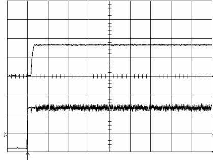
Start-up enabled by connecting V_i at: T_{ref} = +25^{\circ}C , I_o = 50 A resistive load, V_i = 12.0 V. Top trace: output voltage (2.0 V/div.). Bottom trace: input voltage (5 V/div.). Time scale: 20 ms/div.
