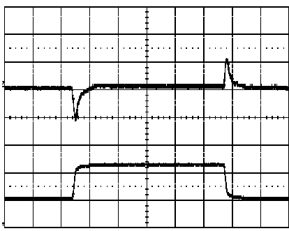
Output voltage response to load current step- change (25-50-25 A) at: T_{ref} = +25^{\circ}C , V_i = 12.0 V. Top trace: output voltage (100 mV/div.). Bottom trace: load current (20 A/div.). Time scale: 0.2 ms/div.
