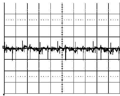
Output voltage ripple (20 mV/div.) at: T_{ref} = +25^\circ\text{C} , I_o = 50\text{ A} resistive load, V_i = 12.0\text{ V} . Time scale: 2 \mu\text{s} /div. See the filter in the Output ripple and noise section (EMC Specification).
