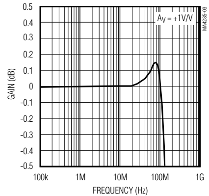
MAX4285/MAX4387/MAX4288 GAIN FLATNESS vs. FREQUENCY ( R_{LOAD} = 100\Omega )
