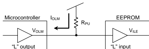
Figure 49. Pull up resistance
