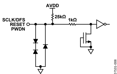
Figure 17. Equivalent SCLK/DFS, RESET, PWDN Input Circuit
