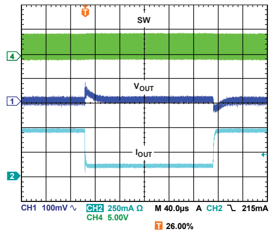
Figure 14. Response to Load Transient, 150 mA to 500 mA, V_{OUT} = 1.8V
