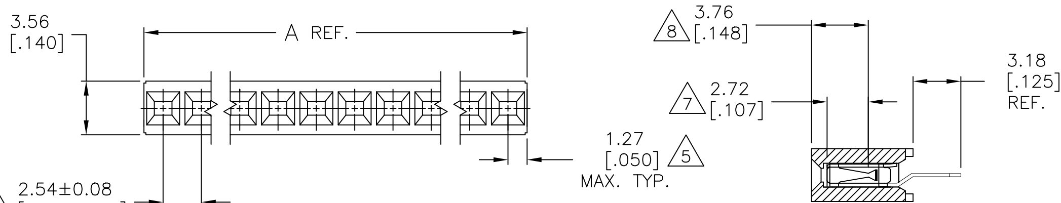
SECTION X-X
