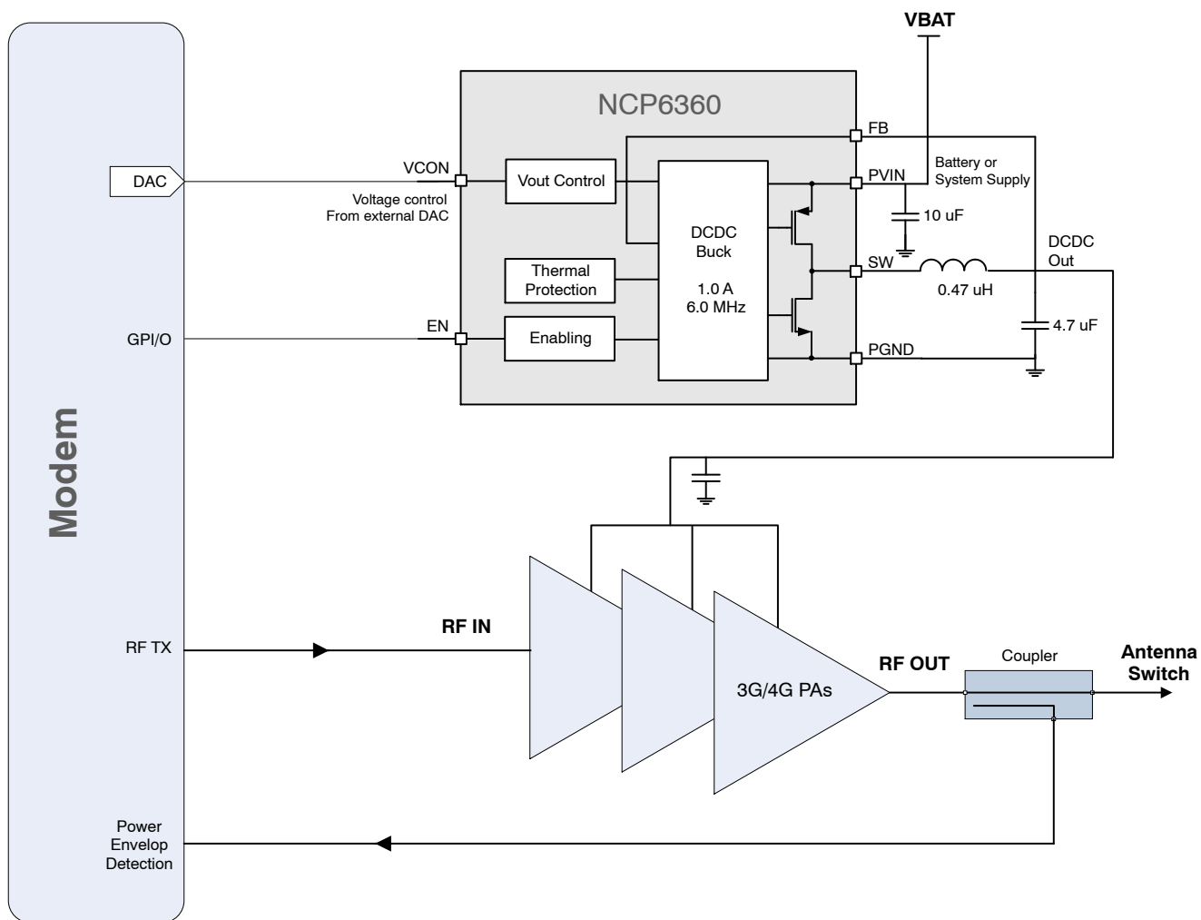
Figure 2. Typical Application
