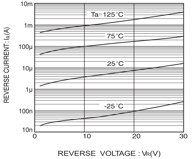
Fig. 2 Reverse characteristics
