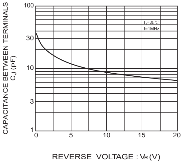
Fig. 3 Capacitance Characteristics
