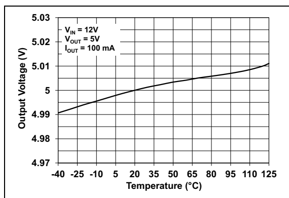
FIGURE 2-12: V_{OUT} vs. Temperature.
