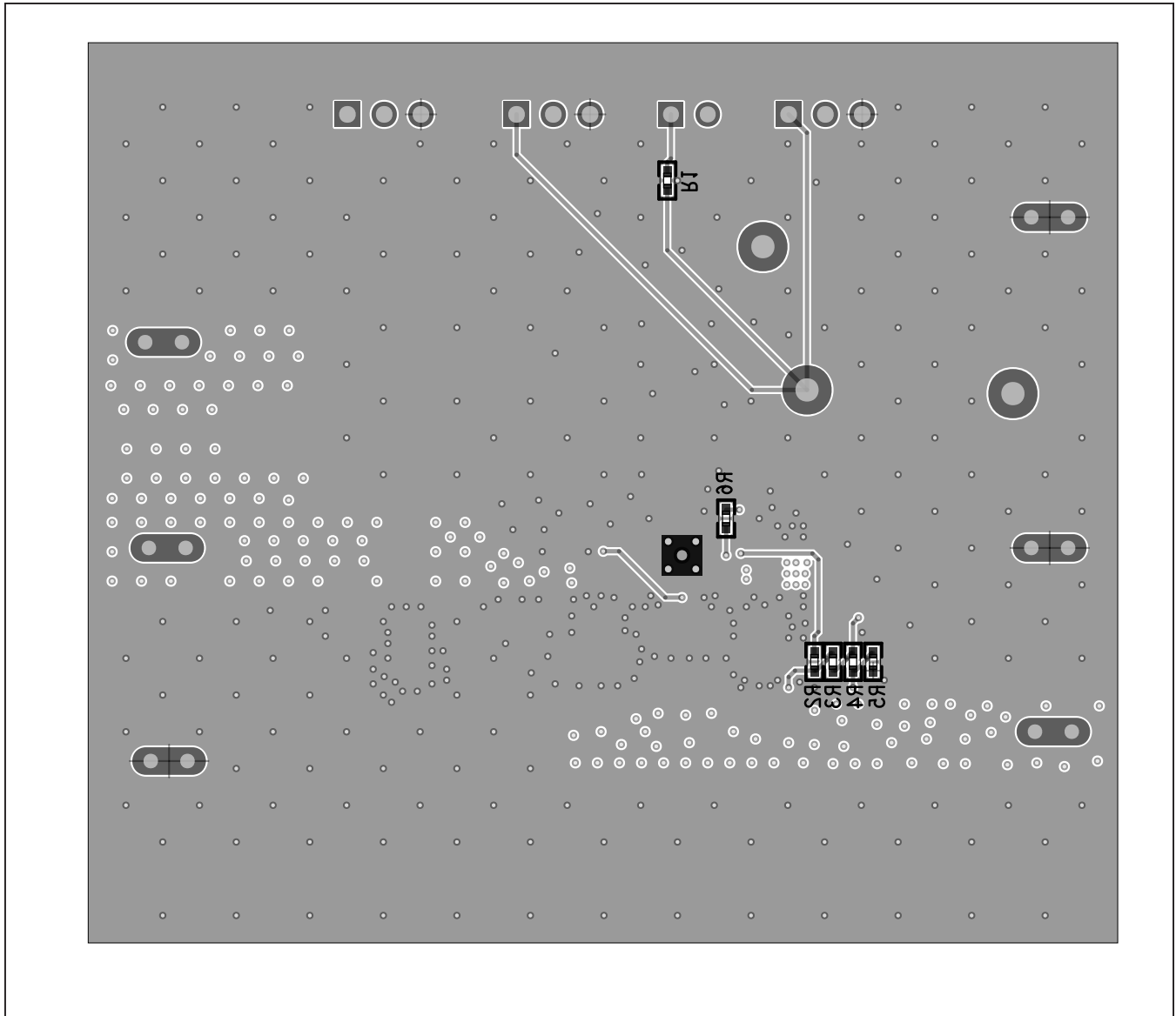
MAX20079 EVKIT Component Placement Guide Bottom
