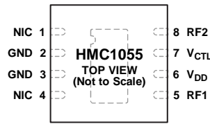
Figure 2. Pin Configuration
