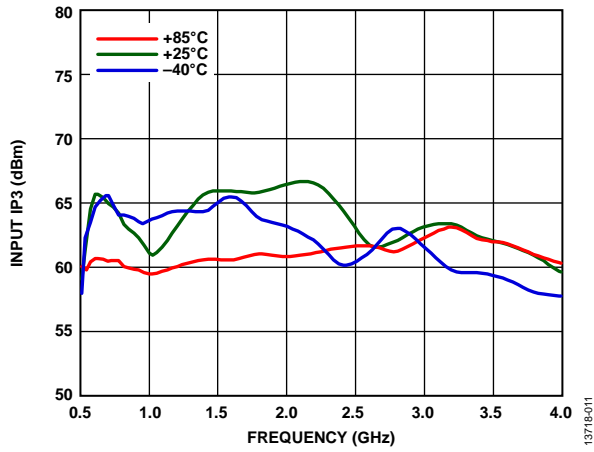
Figure 11. Input IP3 vs. Frequency Over Temperature, V_{DD} = 3 V , V_{CTL} = 3 V
