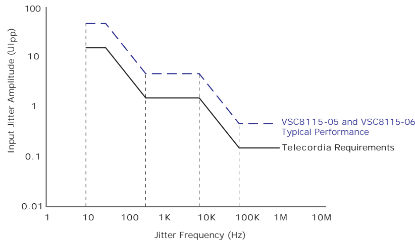
OC-3 Jitter Tolerance Minimum Specifications
