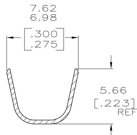
SECTION C-C
