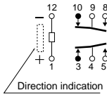
(Deenergized condition)
