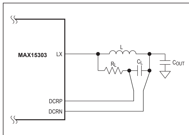
Figure 9. Lossless DCR Current Sensing
