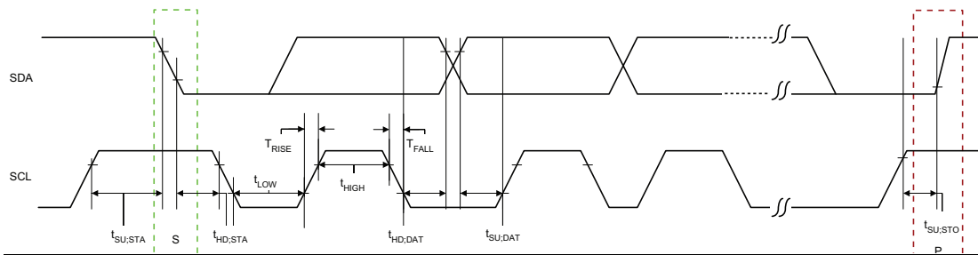
Figure 16 • I²C Timing Parameter Definition
