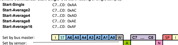
Figure 3 - I2C Communication Diagram
