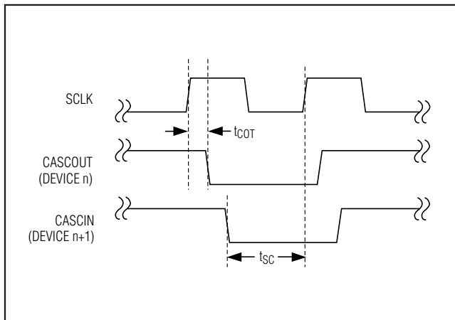
Figure 9. CASCIN and CASCOUT Timing Diagram
