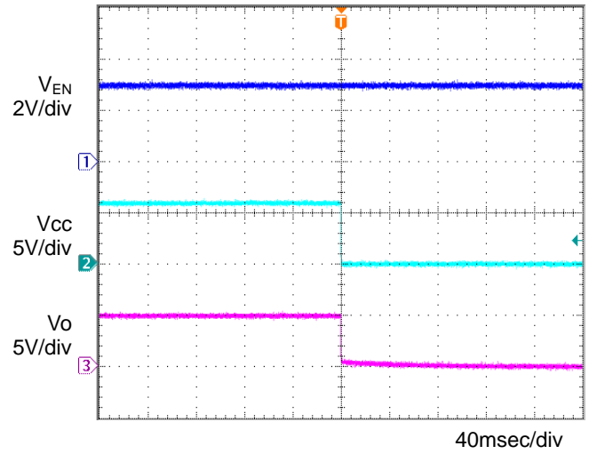
Figure 12. OFF sequence 1 C_o = 1\mu\text{F} , T_a = -40^\circ\text{C}
