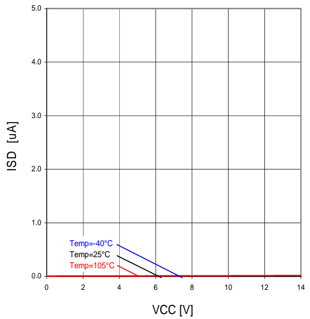
Figure 26. V_{CC}-I_{SD} ( V_{EN}=0V )
