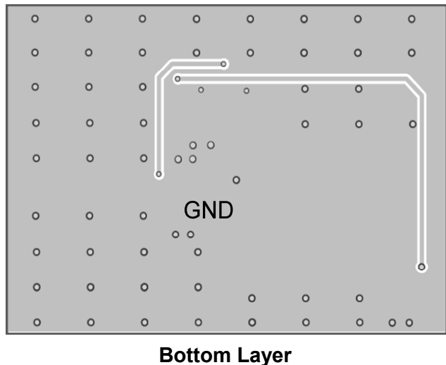
Figure 7: Recommended PCB Layout
