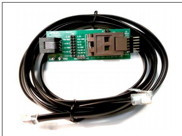
Figure 1. DS9120P EV Board with RJ11 Cable
