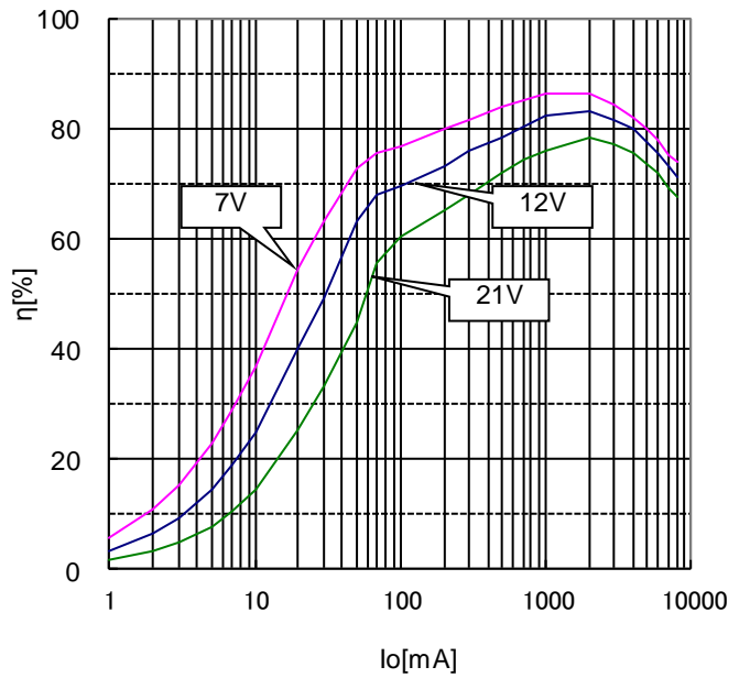
Figure 23. Efficiency (Vo= 1V, QLLM)
