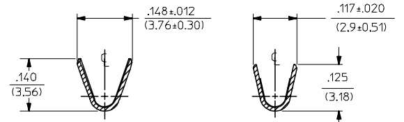
SECT. "A-A"
