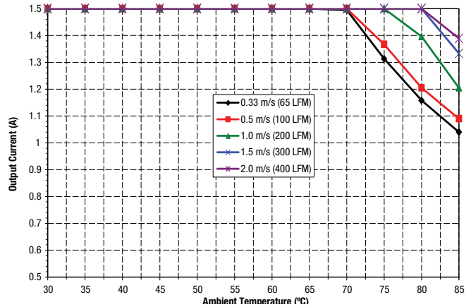
Maximum Current Temperature Derating at Sea Level ( V_{IN} = 24V , airflow is from pin 1 to pin 4)
