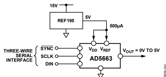
Figure 36. REF195 as Power Supply to the AD5663
