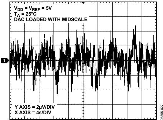
Figure 23. 0.1 Hz to 10 Hz Output Noise Plot
