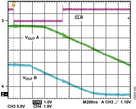
Figure 26. CLR Pulse Activation Time
