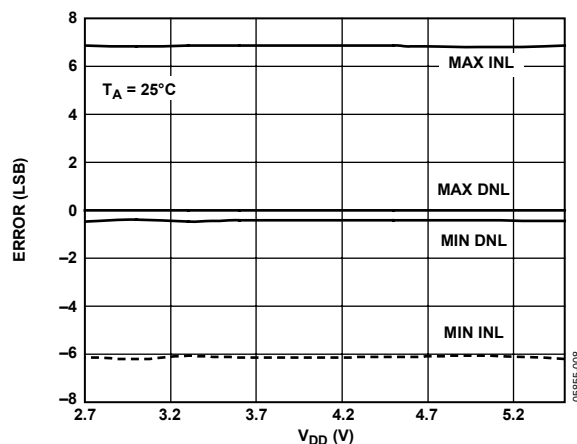
Figure 8. INL and DNL Error vs. Supply
