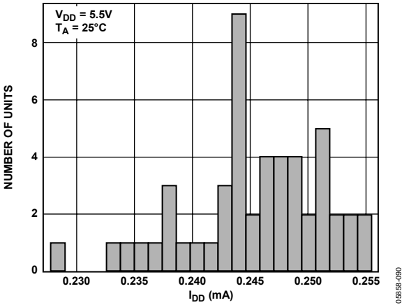
Figure 13. I_{DD} Histogram with V_{DD} = 5.5 V
