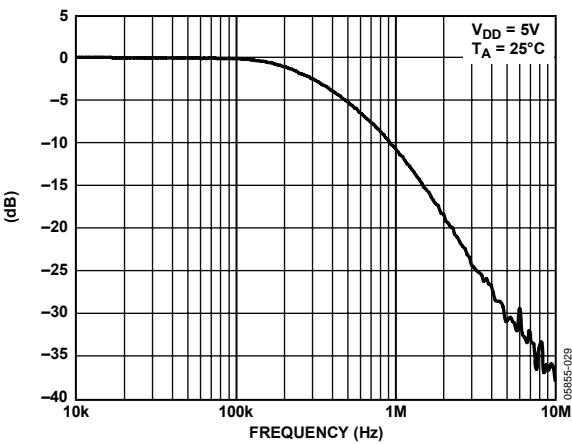
Figure 25. Multiplying Bandwidth
