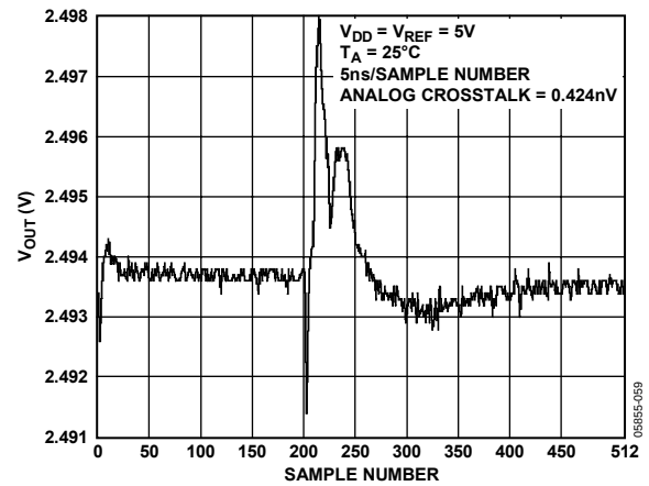
Figure 20. Analog Crosstalk
