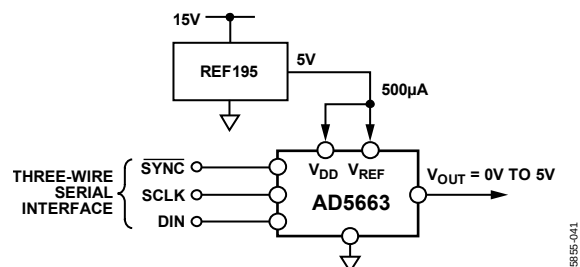
Figure 36. REF195 as Power Supply to the AD5663
